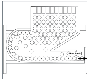
Can Flow Diagram
