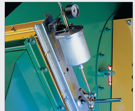
Damper Adjustment
