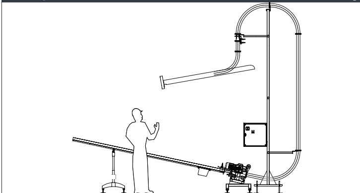
Drawing of Fleetwood Manual Can Lid Feeder with LLV Low Level V-Tray
